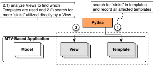
Figure 2: In the Model Template View (MTV) Context, Pythia focuses on Views and Templates.
