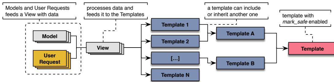
Figure 1: A potentially vulnerable Django template is included by various templates which in turn are utilized by Django Views
